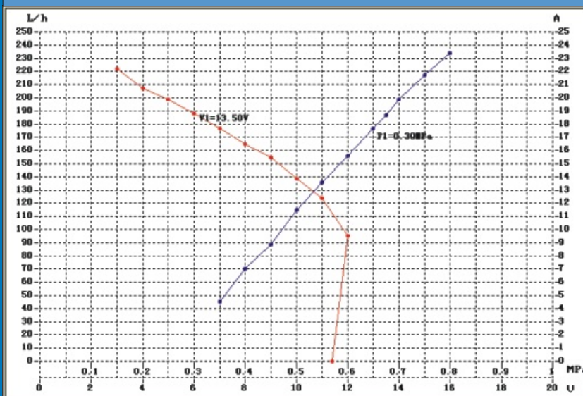
A CHR Electric Fuel Pump L = f(P) L = f(V) Test Report
