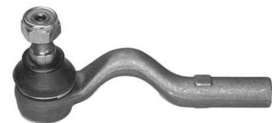
▶ Orj Ref : MCD64-L Descr. : Tie rod end-L OEM No : 2103380615 Note : M14*1.5 RHT
