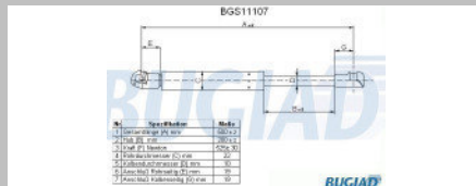
Gas Spring
