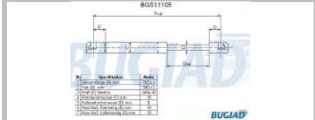
Gas Spring
